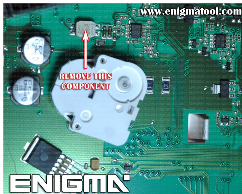
PHOTO 1: Disassemble the dash to get to the component shown on the photo above.
