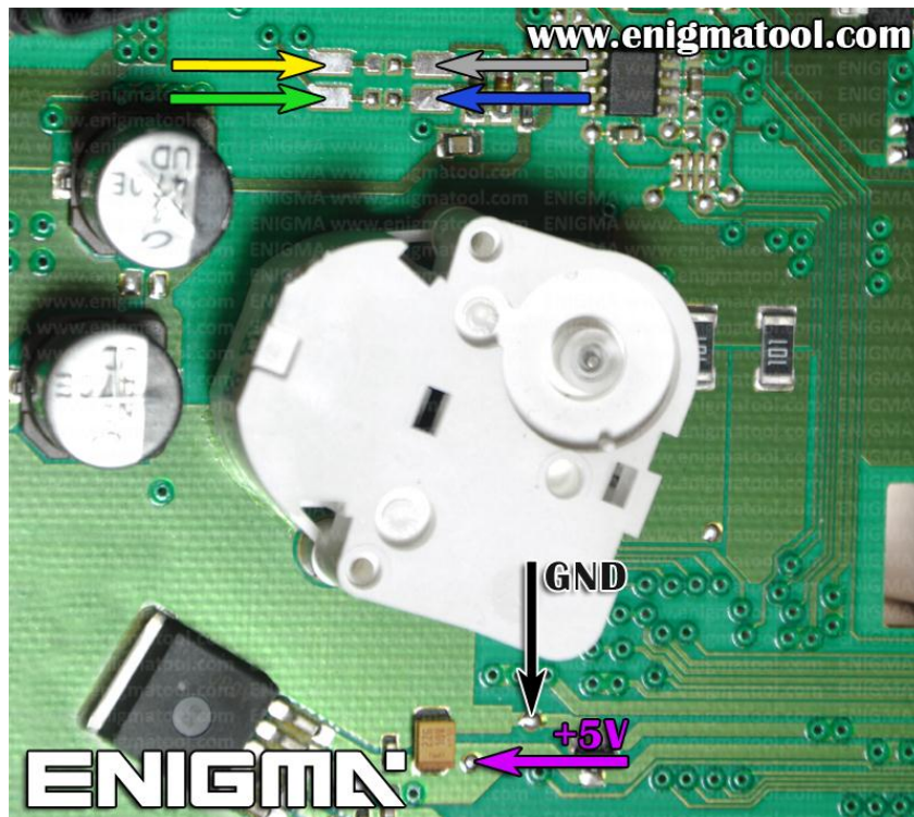
PHOTO 2: Solder cables according to the colors like shown on the photo above.
