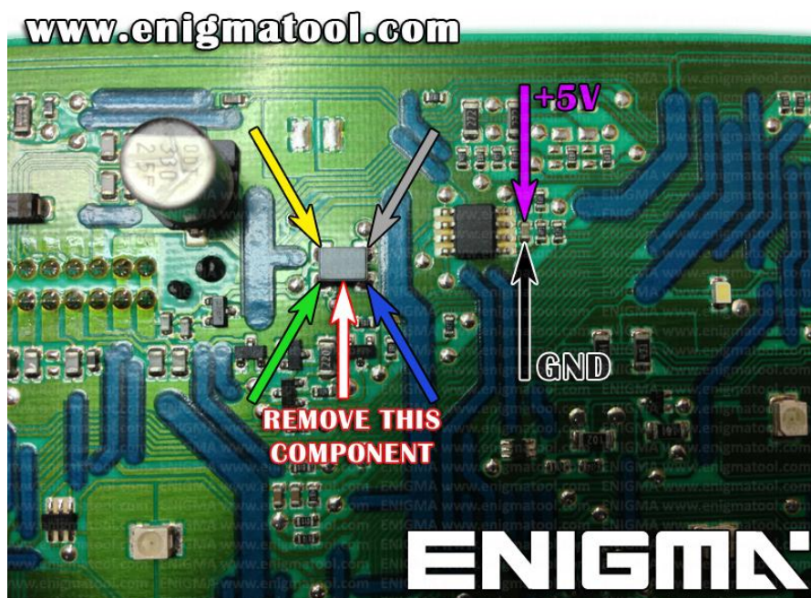
PHOTO 1: Remove component and solder cables according to the colors like shown on the photo above.
